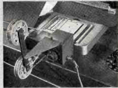
Coming events, time and news tapes and commercials receive smooth treatment on large capacity roll-thru carriages.
